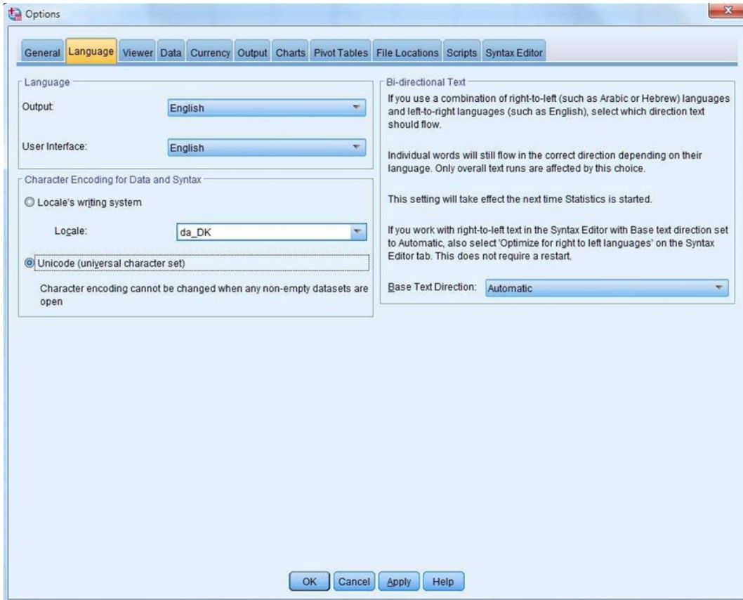
Figur 3 Fanebladet "Language" under Options i SPSS
